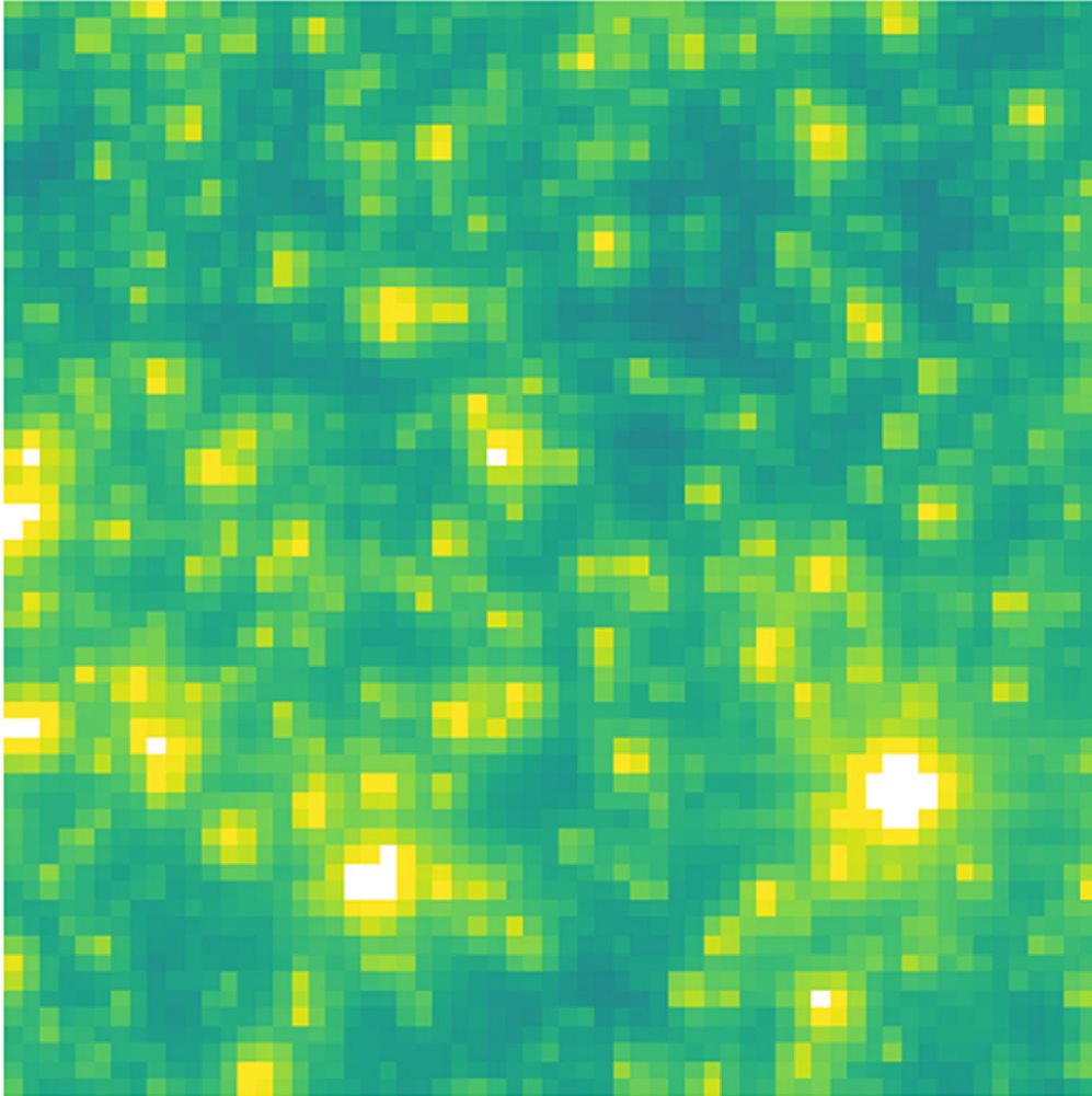
Figure 3. from Michael D. Albrow 2025 Astron. J. 169 doi:10.3847/1538-3881/adc9a1 https://dx.doi.org/10.3847/1538-3881/adc9a1 © 2025. The Author(s). Published by the American Astronomical Society.
