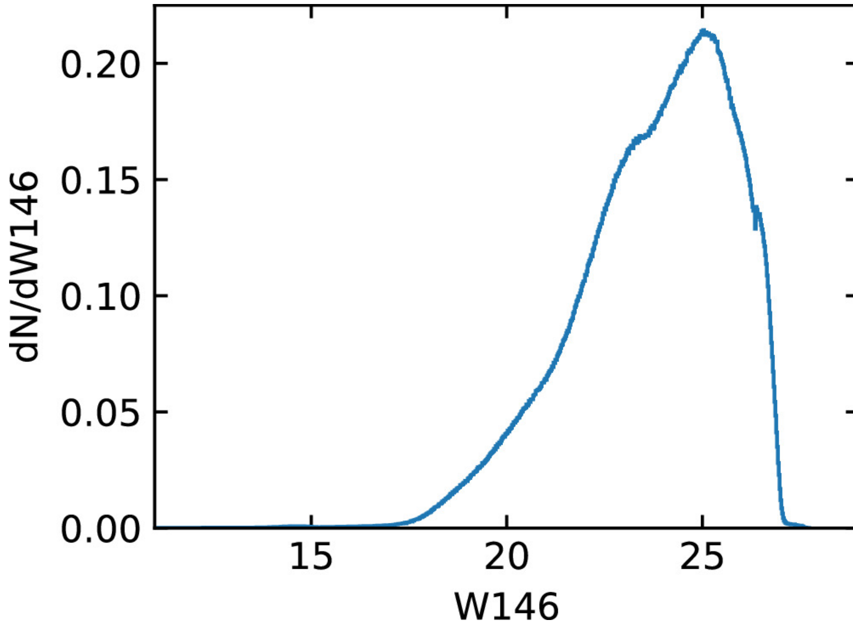
Figure 2. from Michael D. Albrow 2025 Astron. J. 169 doi:10.3847/1538-3881/adc9a1 https://dx.doi.org/10.3847/1538-3881/adc9a1 © 2025. The Author(s). Published by the American Astronomical Society.
