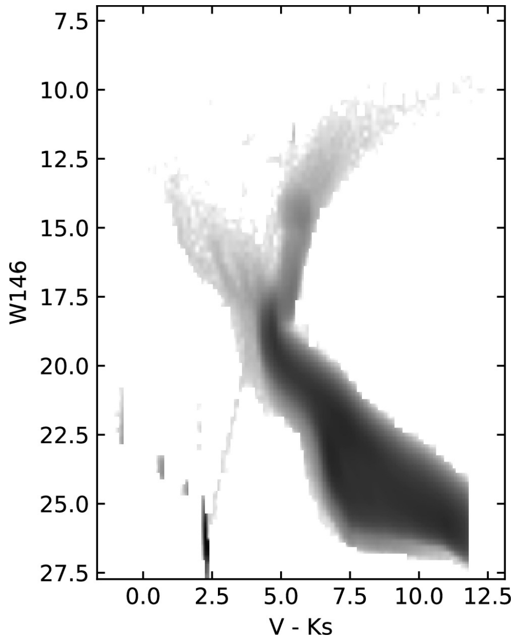
Figure 1. from Michael D. Albrow 2025 Astron. J. 169 doi:10.3847/1538-3881/adc9a1 https://dx.doi.org/10.3847/1538-3881/adc9a1 © 2025. The Author(s). Published by the American Astronomical Society.
