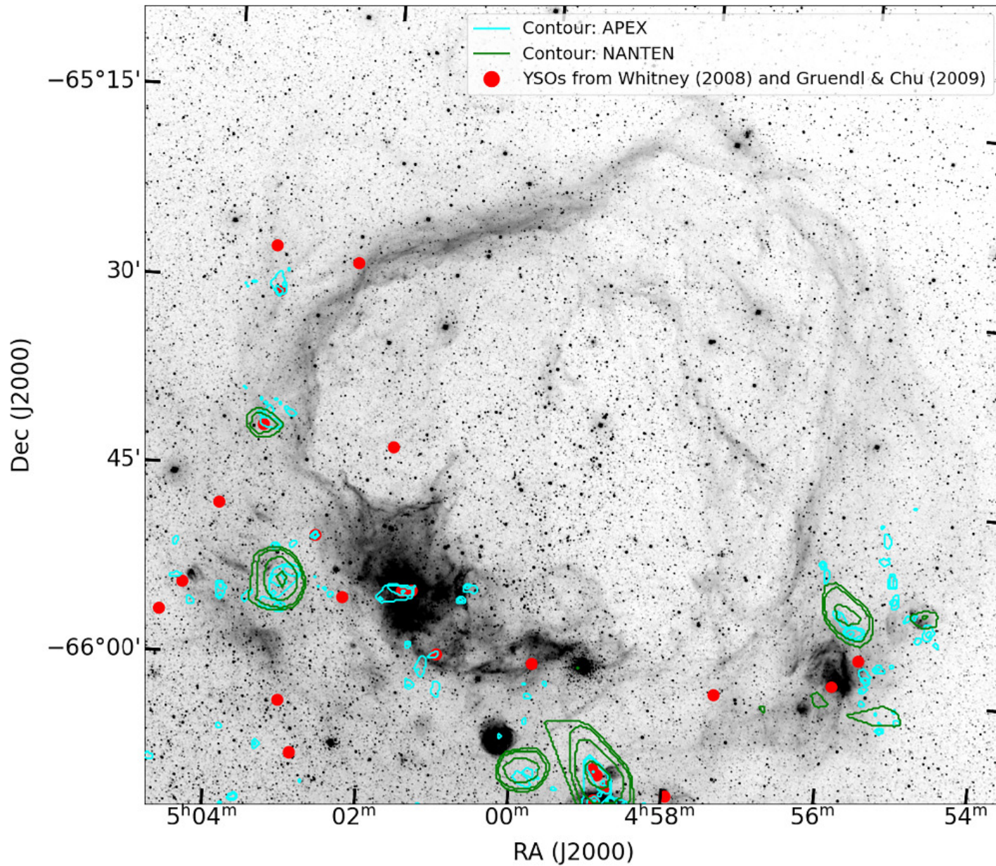
Figure 6. from Guan-Hong Li et al 2025 Astron. J. 169 doi:10.3847/1538-3881/adc90f https://dx.doi.org/10.3847/1538-3881/adc90f © 2025. The Author(s). Published by the American Astronomical Society.
