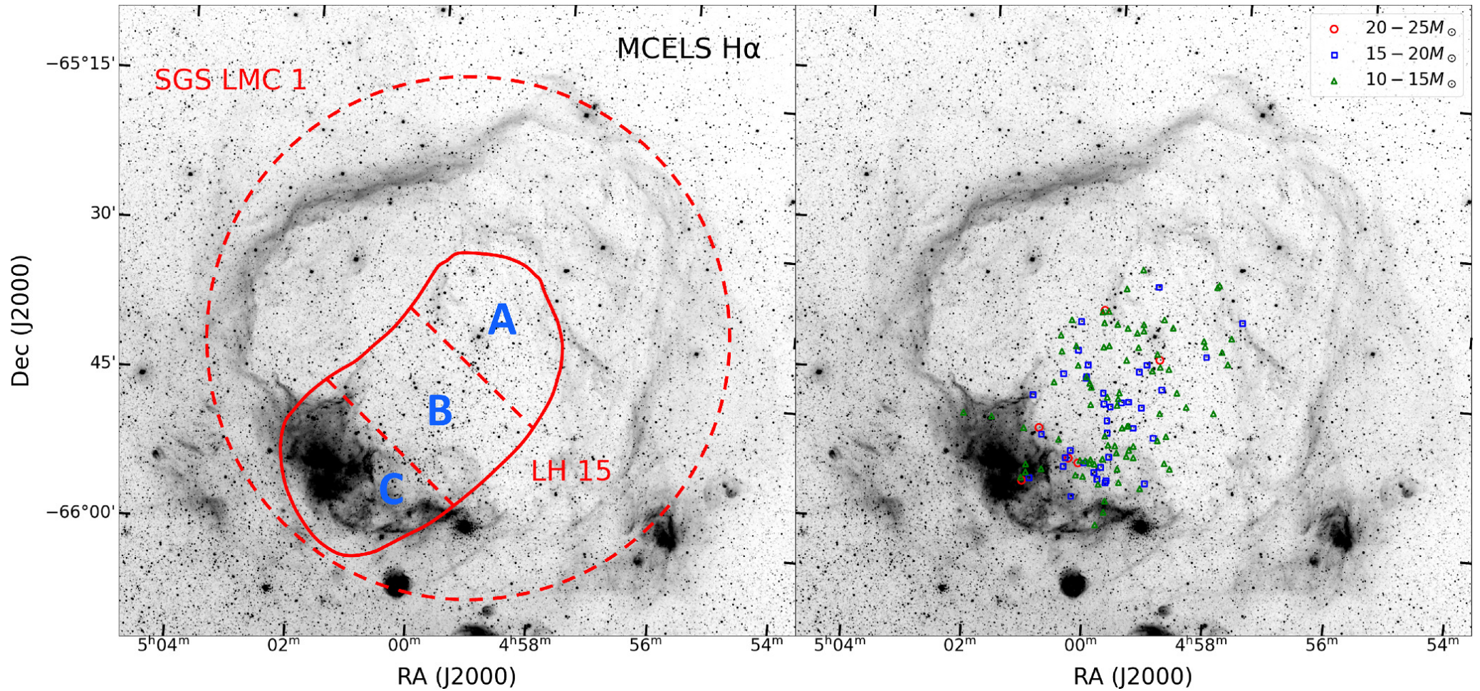
Figure 2. from Guan-Hong Li et al 2025 Astron. J. 169 doi:10.3847/1538-3881/adc90f https://dx.doi.org/10.3847/1538-3881/adc90f © 2025. The Author(s). Published by the American Astronomical Society.
