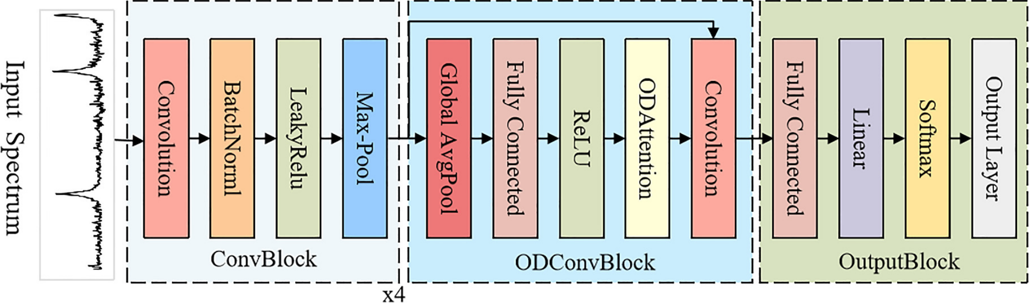
Figure 2. from ZhiWei Lu et al 2025 Astron. J. 169 doi:10.3847/1538-3881/adc738 https://dx.doi.org/10.3847/1538-3881/adc738 © 2025. The Author(s). Published by the American Astronomical Society.
