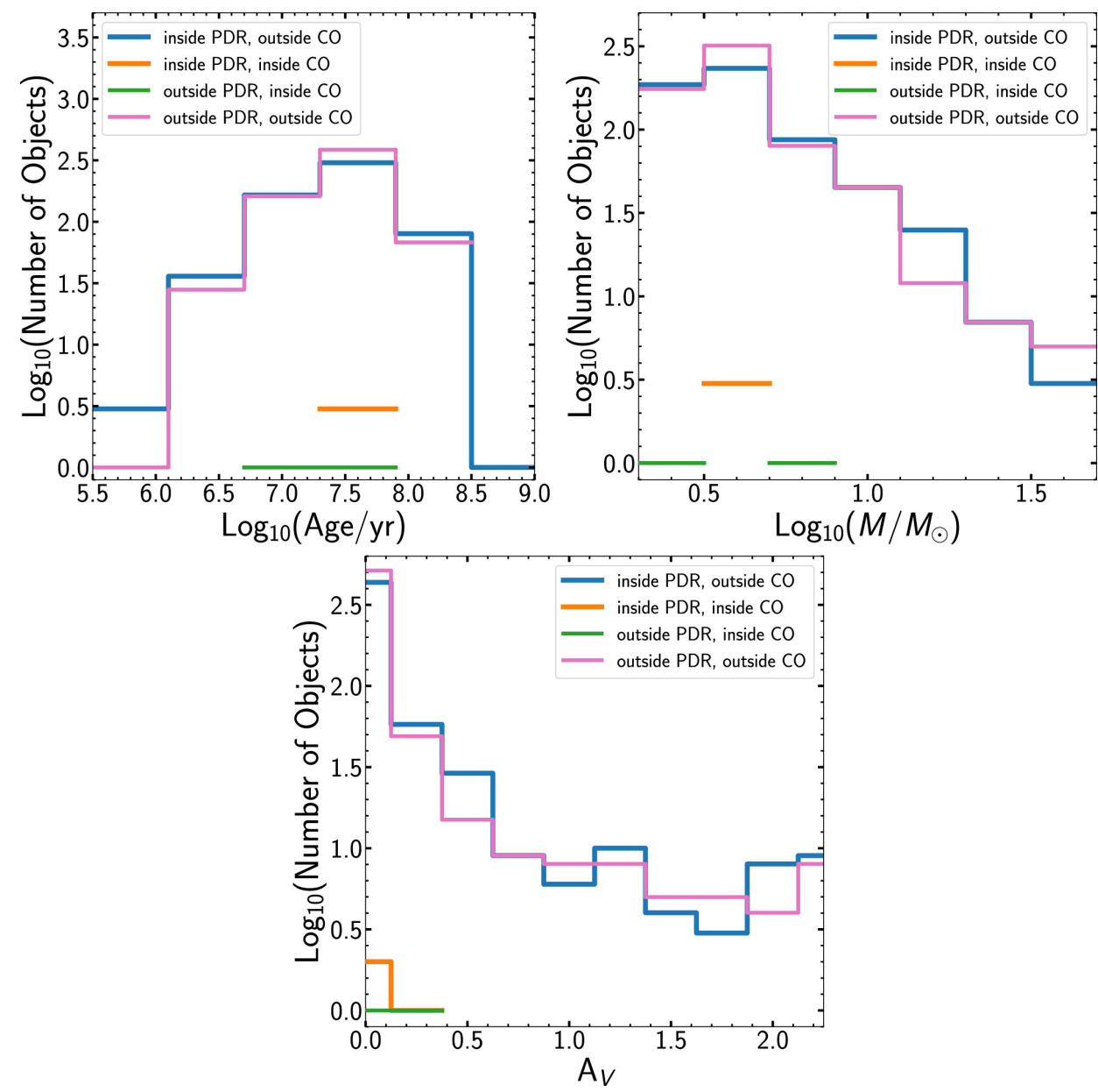
Figure 7. from Haylee N. Archer et al 2025 Astron. J. 169 doi:10.3847/1538-3881/adc736 https://dx.doi.org/10.3847/1538-3881/adc736 © 2025. The Author(s). Published by the American Astronomical Society.
