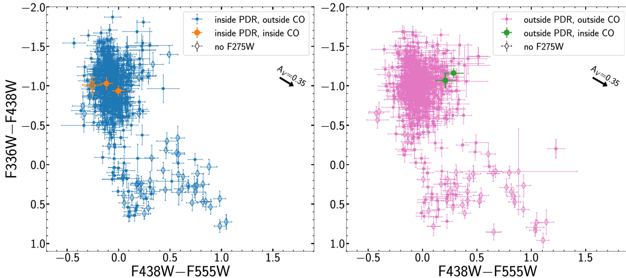
Figure 6. from Haylee N. Archer et al 2025 Astron. J. 169 doi:10.3847/1538-3881/adc736 https://dx.doi.org/10.3847/1538-3881/adc736 © 2025. The Author(s). Published by the American Astronomical Society.
