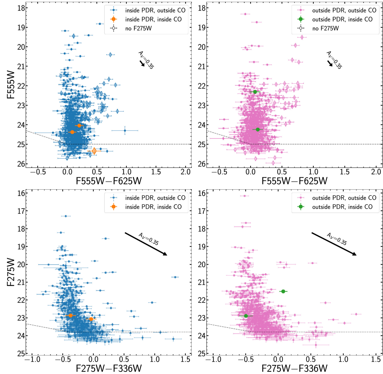
Figure 5. from Haylee N. Archer et al 2025 Astron. J. 169 doi:10.3847/1538-3881/adc736 https://dx.doi.org/10.3847/1538-3881/adc736 © 2025. The Author(s). Published by the American Astronomical Society.
