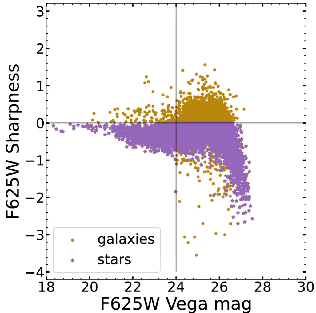
Figure 4. from Haylee N. Archer et al 2025 Astron. J. 169 doi:10.3847/1538-3881/adc736 https://dx.doi.org/10.3847/1538-3881/adc736 © 2025. The Author(s). Published by the American Astronomical Society.
