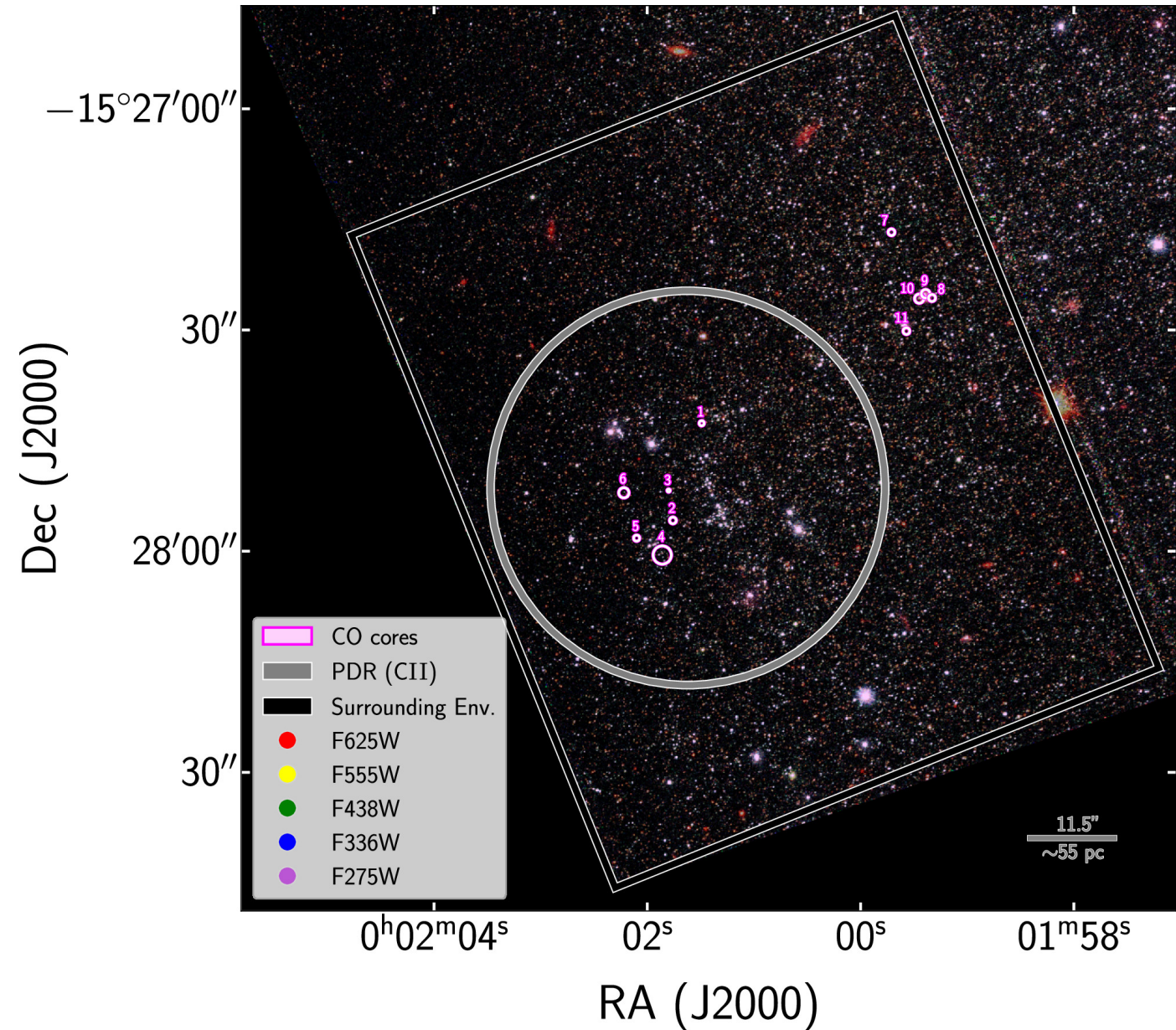
Figure 1. from Haylee N. Archer et al 2025 Astron. J. 169 doi:10.3847/1538-3881/adc736 https://dx.doi.org/10.3847/1538-3881/adc736 © 2025. The Author(s). Published by the American Astronomical Society.
