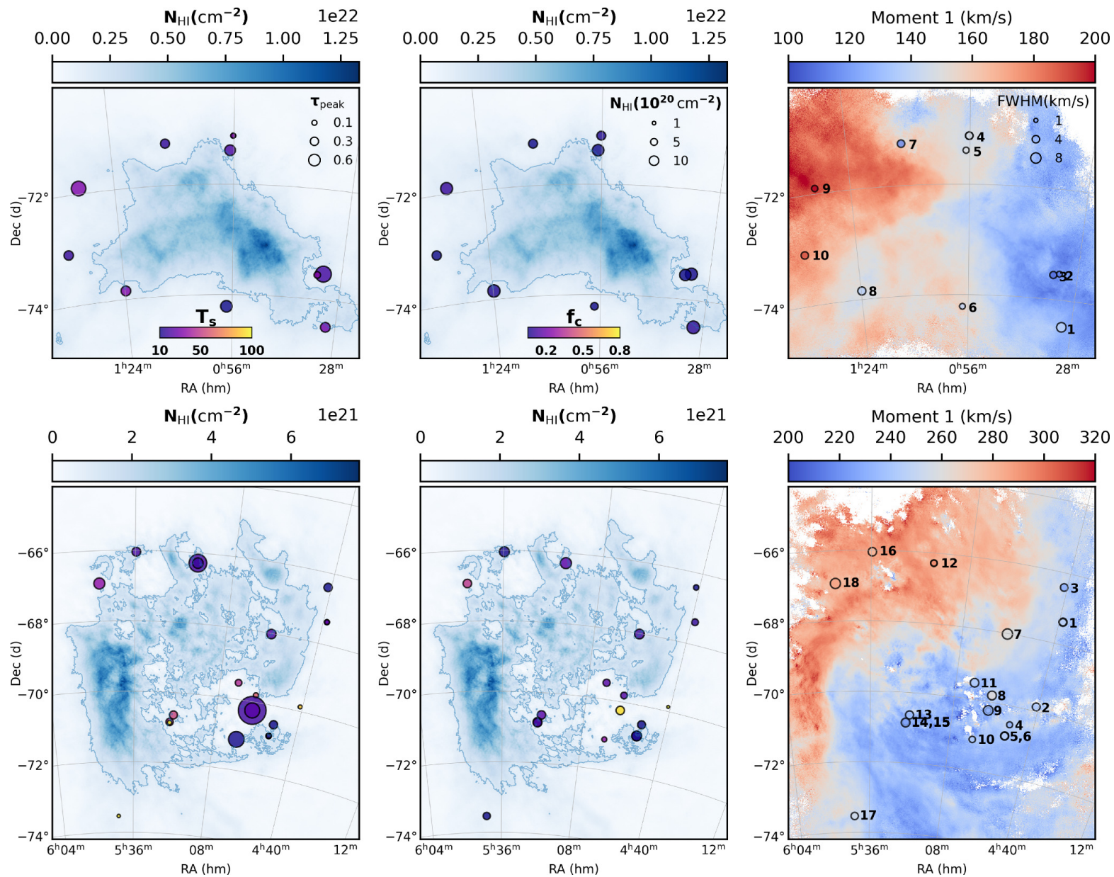
Figure 6. from Hongxing Chen et al 2025 Astron. J. 169 doi:10.3847/1538-3881/adc67c https://dx.doi.org/10.3847/1538-3881/adc67c © 2025. The Author(s). Published by the American Astronomical Society.
