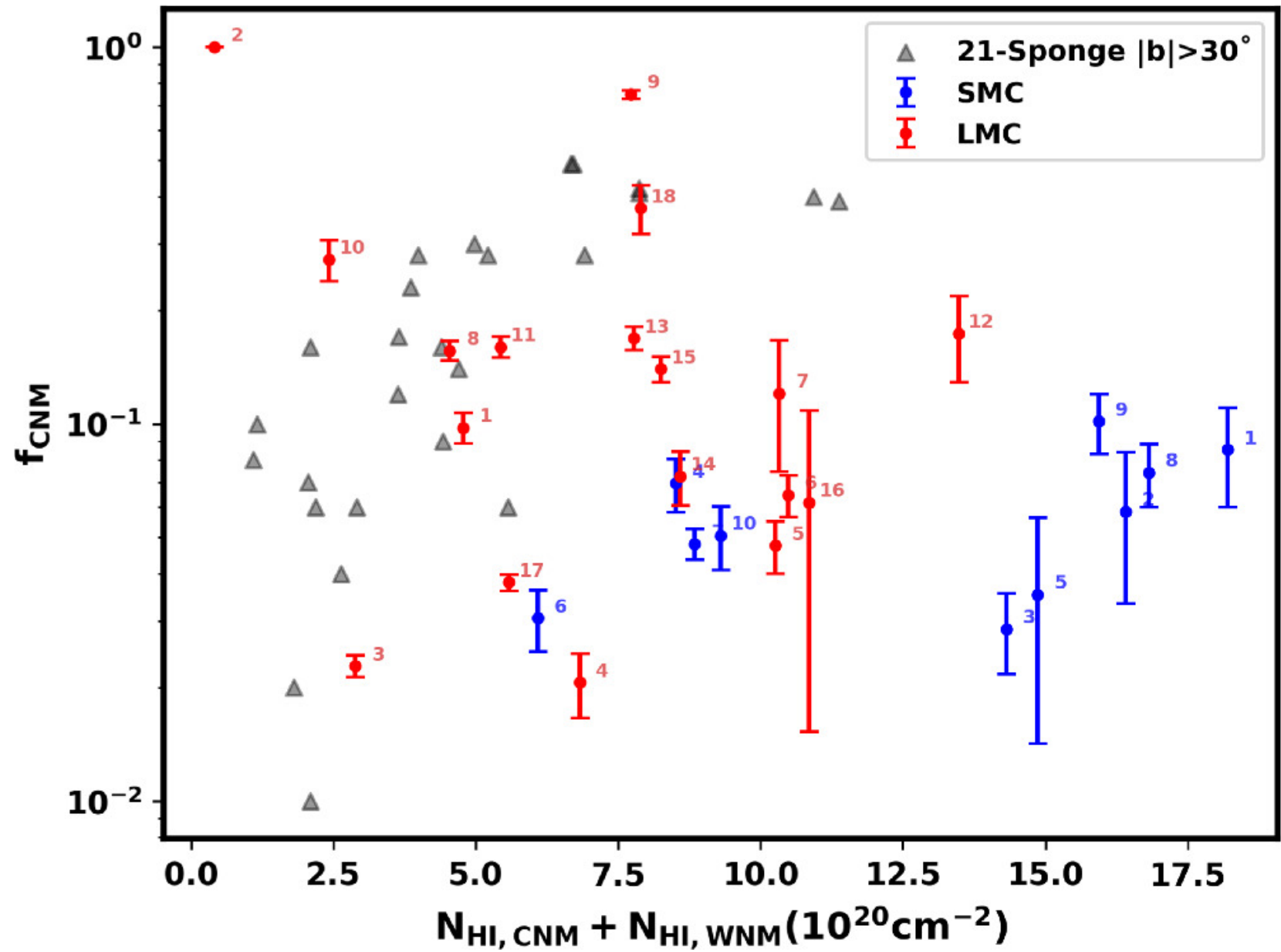
Figure 5. from Hongxing Chen et al 2025 Astron. J. 169 doi:10.3847/1538-3881/adc67c https://dx.doi.org/10.3847/1538-3881/adc67c © 2025. The Author(s). Published by the American Astronomical Society.
