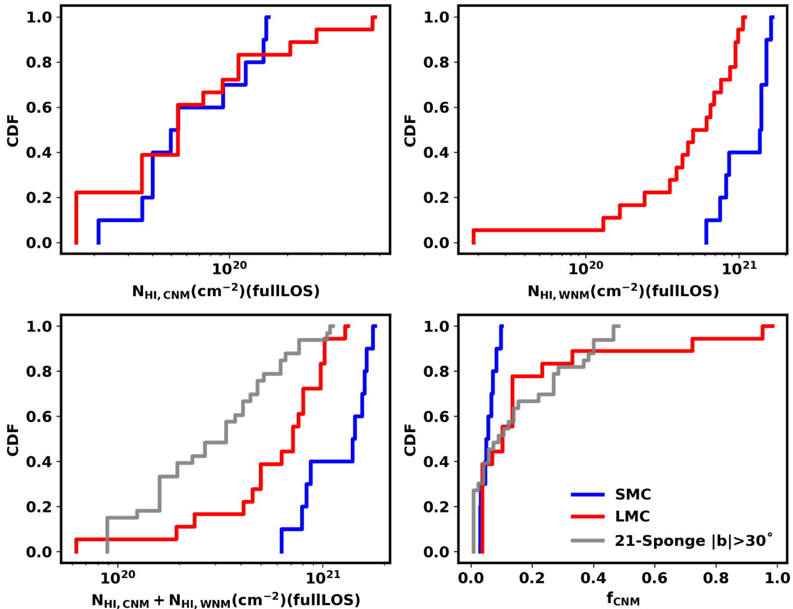
Figure 4. from Hongxing Chen et al 2025 Astron. J. 169 doi:10.3847/1538-3881/adc67c https://dx.doi.org/10.3847/1538-3881/adc67c © 2025. The Author(s). Published by the American Astronomical Society.
