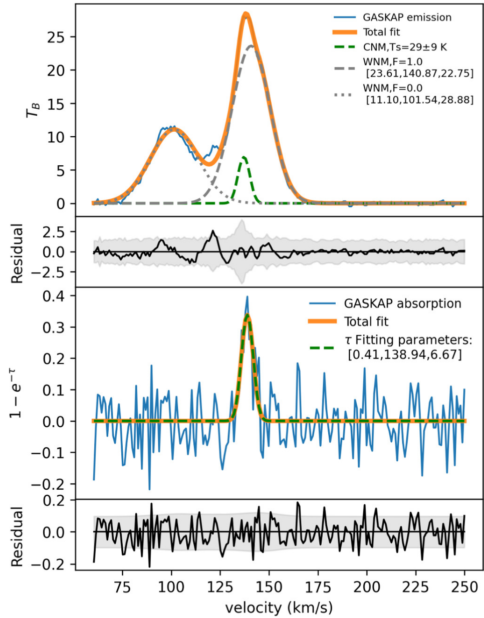
Figure 2. from Hongxing Chen et al 2025 Astron. J. 169 doi:10.3847/1538-3881/adc67c https://dx.doi.org/10.3847/1538-3881/adc67c © 2025. The Author(s). Published by the American Astronomical Society.
