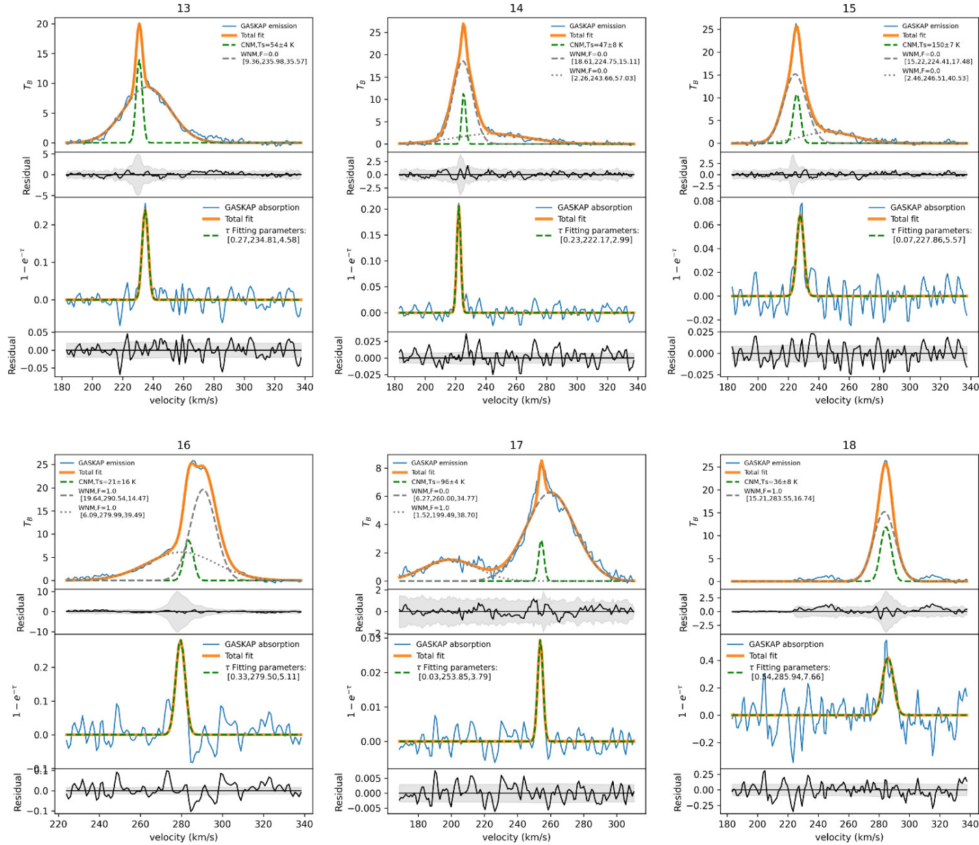
Figure 10. from Hongxing Chen et al 2025 Astron. J. 169 doi:10.3847/1538-3881/adc67c https://dx.doi.org/10.3847/1538-3881/adc67c © 2025. The Author(s). Published by the American Astronomical Society.
