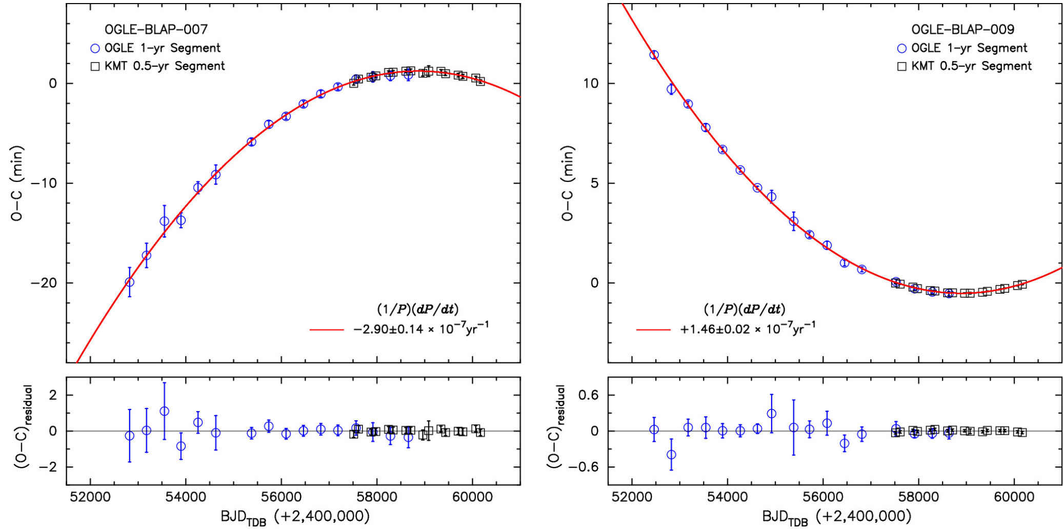
Figure 8. from Seung-Lee Kim et al 2025 Astron. J. 169 doi:10.3847/1538-3881/adc4e4 https://dx.doi.org/10.3847/1538-3881/adc4e4 © 2025. The Author(s). Published by the American Astronomical Society.
