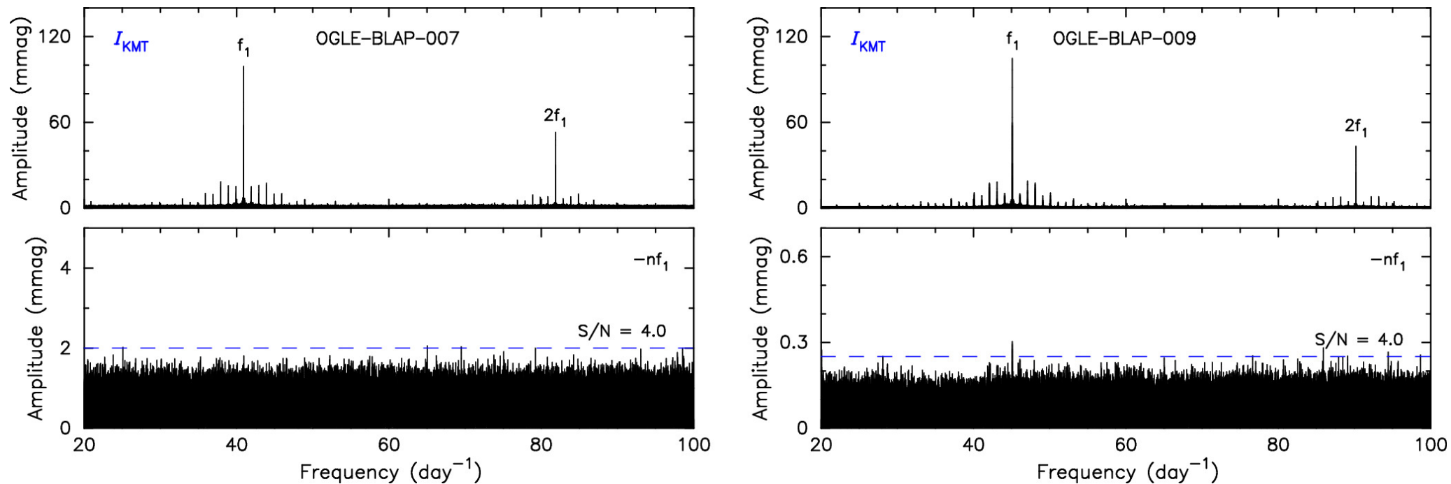
Figure 7. from Seung-Lee Kim et al 2025 Astron. J. 169 doi:10.3847/1538-3881/adc4e4 https://dx.doi.org/10.3847/1538-3881/adc4e4 © 2025. The Author(s). Published by the American Astronomical Society.
