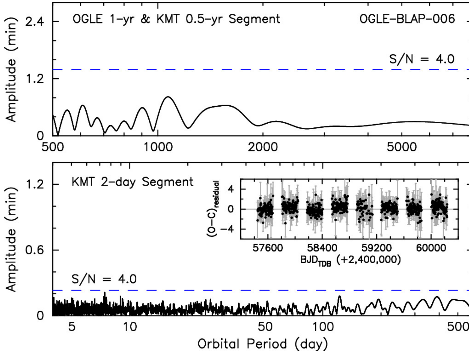
Figure 5. from Seung-Lee Kim et al 2025 Astron. J. 169 doi:10.3847/1538-3881/adc4e4 https://dx.doi.org/10.3847/1538-3881/adc4e4 © 2025. The Author(s). Published by the American Astronomical Society.
