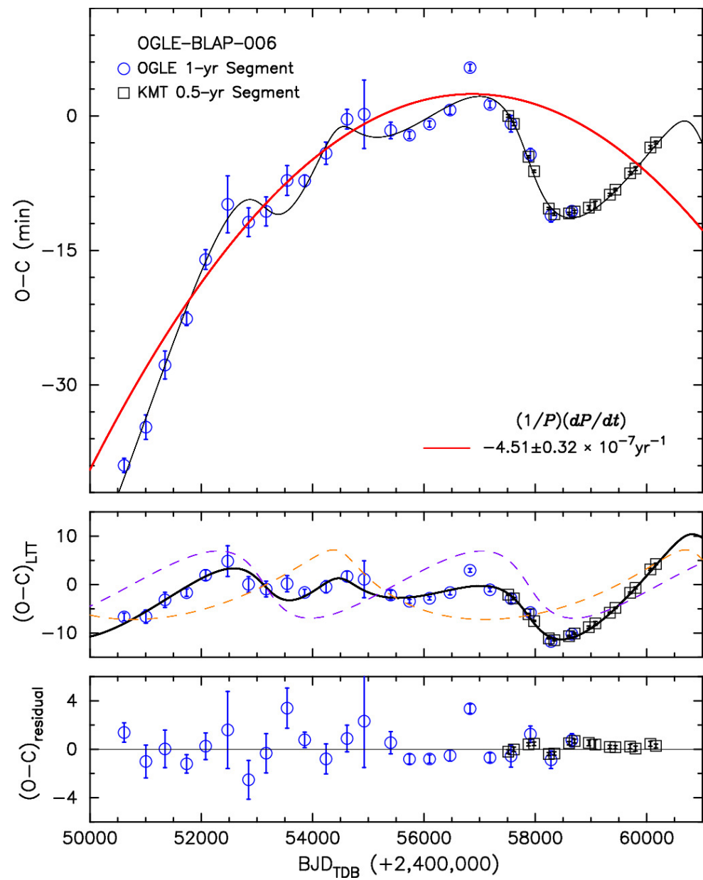
Figure 4. from Seung-Lee Kim et al 2025 Astron. J. 169 doi:10.3847/1538-3881/adc4e4 https://dx.doi.org/10.3847/1538-3881/adc4e4 © 2025. The Author(s). Published by the American Astronomical Society.
