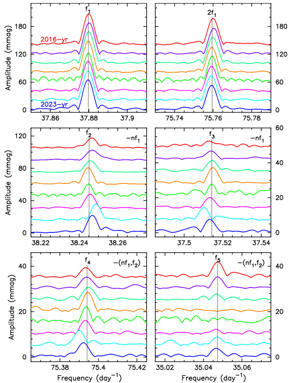
Figure 3. from Seung-Lee Kim et al 2025 Astron. J. 169 doi:10.3847/1538-3881/adc4e4 https://dx.doi.org/10.3847/1538-3881/adc4e4 © 2025. The Author(s). Published by the American Astronomical Society.
