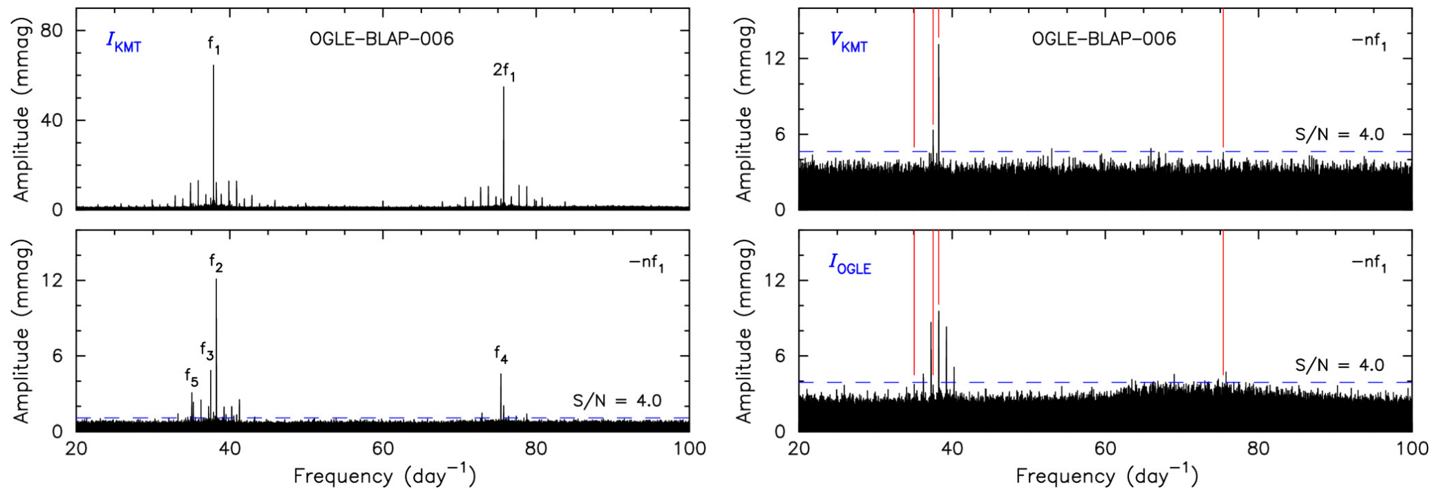
Figure 2. from Seung-Lee Kim et al 2025 Astron. J. 169 doi:10.3847/1538-3881/adc4e4 https://dx.doi.org/10.3847/1538-3881/adc4e4 © 2025. The Author(s). Published by the American Astronomical Society.
