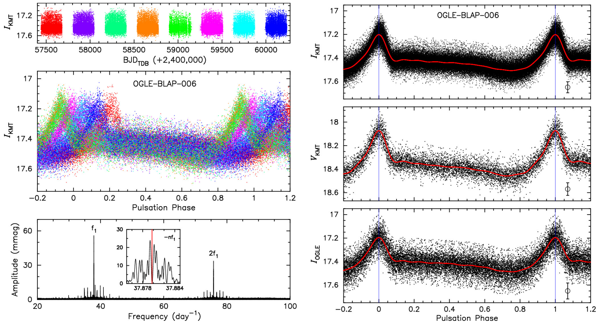
Figure 1. from Seung-Lee Kim et al 2025 Astron. J. 169 doi:10.3847/1538-3881/adc4e4 https://dx.doi.org/10.3847/1538-3881/adc4e4 © 2025. The Author(s). Published by the American Astronomical Society.
