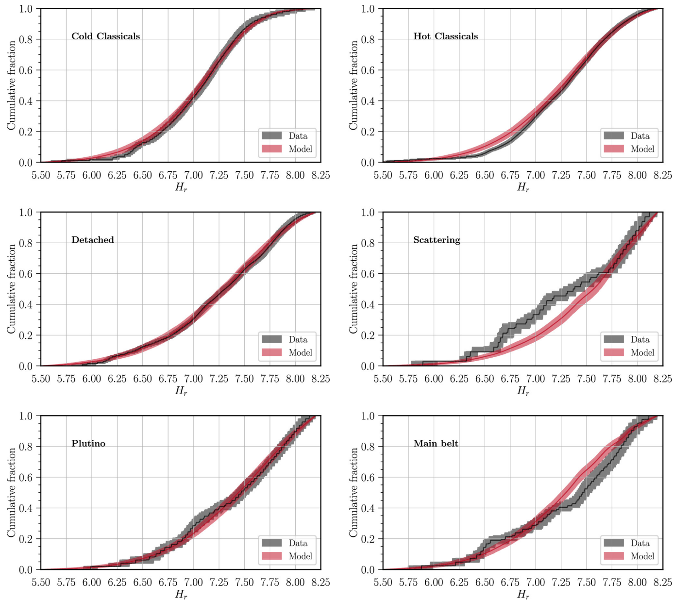
Figure 9. from Pedro H. Bernardinelli et al 2025 Astron. J. 169 doi:10.3847/1538-3881/adc459 https://dx.doi.org/10.3847/1538-3881/adc459 © 2025. The Author(s). Published by the American Astronomical Society.
