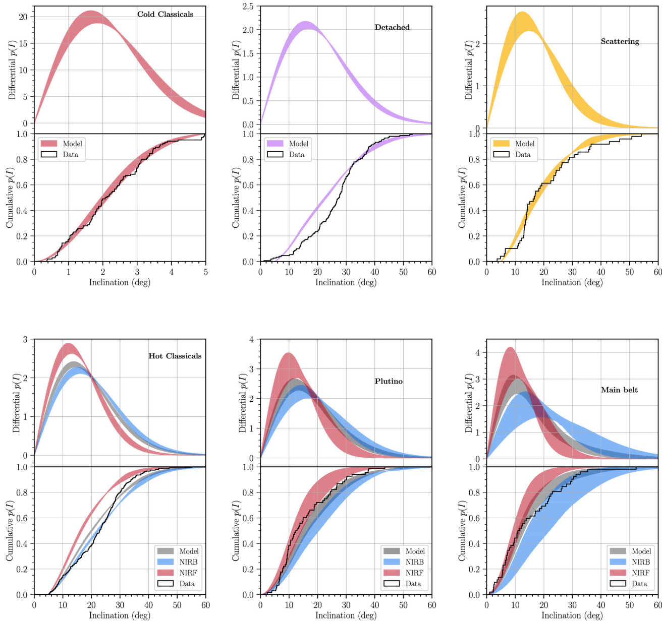
Figure 14. from Pedro H. Bernardinelli et al 2025 Astron. J. 169 doi:10.3847/1538-3881/adc459 https://dx.doi.org/10.3847/1538-3881/adc459 © 2025. The Author(s). Published by the American Astronomical Society.
