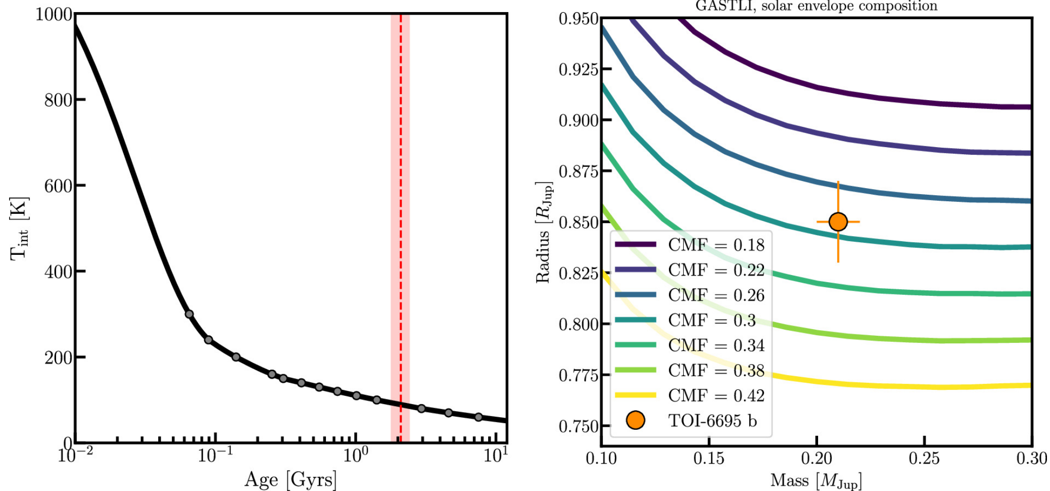
Figure 8. from Jan Eberhardt et al 2025 Astron. J. 169 doi:10.3847/1538-3881/adc44e https://dx.doi.org/10.3847/1538-3881/adc44e © 2025 The Author(s). Published by the American Astronomical Society.
