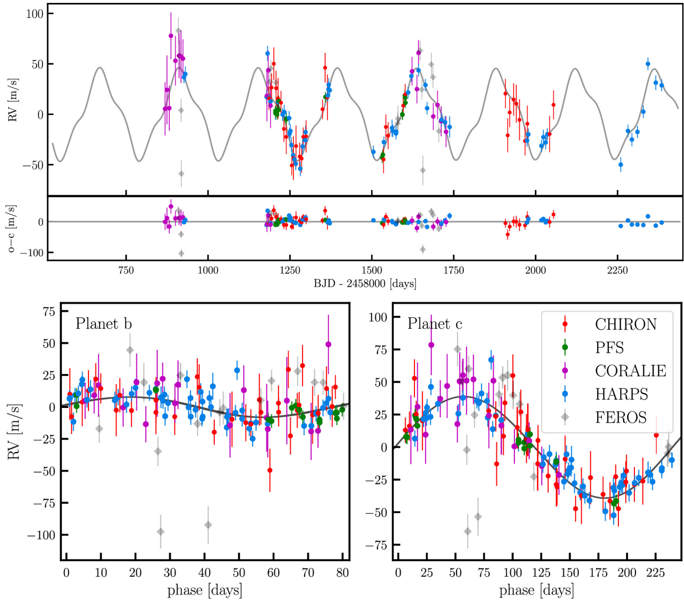
Figure 5. from Jan Eberhardt et al 2025 Astron. J. 169 doi:10.3847/1538-3881/adc44e https://dx.doi.org/10.3847/1538-3881/adc44e © 2025 The Author(s). Published by the American Astronomical Society.
