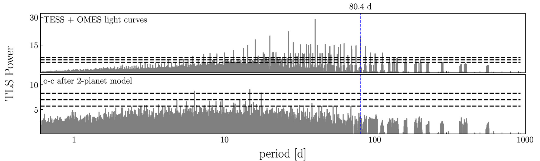
Figure 3. from Jan Eberhardt et al 2025 Astron. J. 169 doi:10.3847/1538-3881/adc44e https://dx.doi.org/10.3847/1538-3881/adc44e © 2025 The Author(s). Published by the American Astronomical Society.
