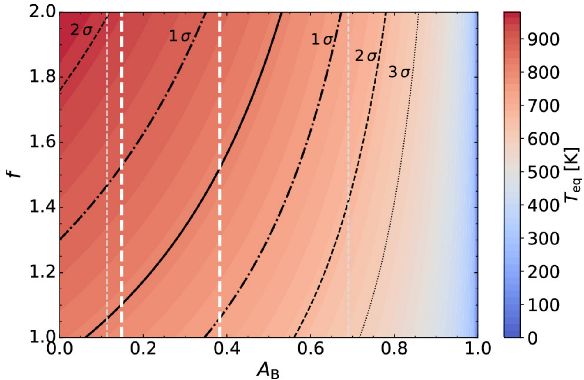
Figure 6. from Kim Morel et al 2025 Astron. J. 169 doi:10.3847/1538-3881/adc43f https://dx.doi.org/10.3847/1538-3881/adc43f © 2025. The Author(s). Published by the American Astronomical Society.
