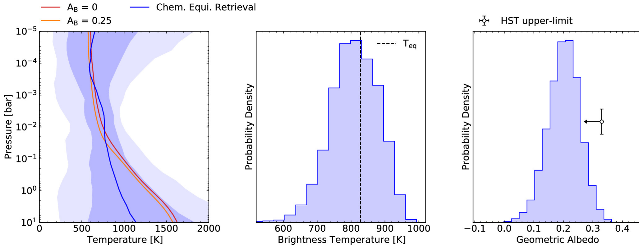
Figure 5. from Kim Morel et al 2025 Astron. J. 169 doi:10.3847/1538-3881/adc43f https://dx.doi.org/10.3847/1538-3881/adc43f © 2025. The Author(s). Published by the American Astronomical Society.
