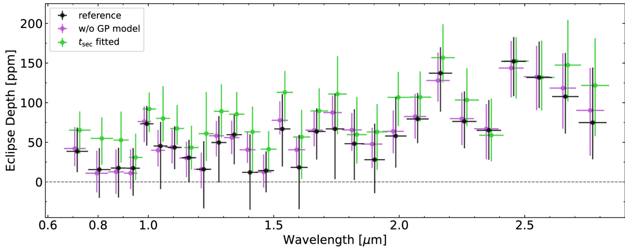
Figure B5. from Kim Morel et al 2025 Astron. J. 169 doi:10.3847/1538-3881/adc43f https://dx.doi.org/10.3847/1538-3881/adc43f © 2025. The Author(s). Published by the American Astronomical Society.
