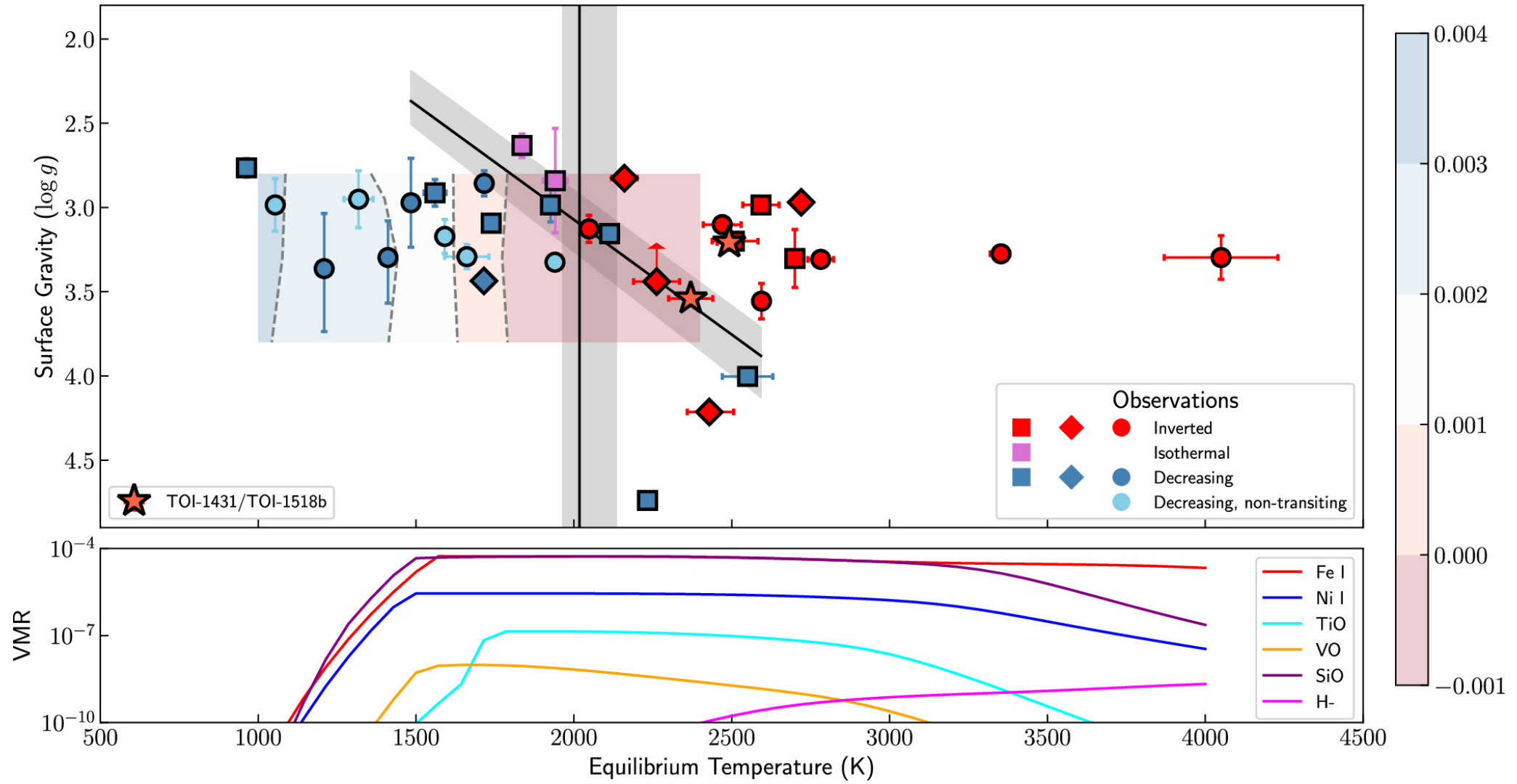
Figure 7. from Sydney Petz et al 2025 Astron. J. 169 doi:10.3847/1538-3881/adc411 https://dx.doi.org/10.3847/1538-3881/adc411 © 2025. The Author(s). Published by the American Astronomical Society.
