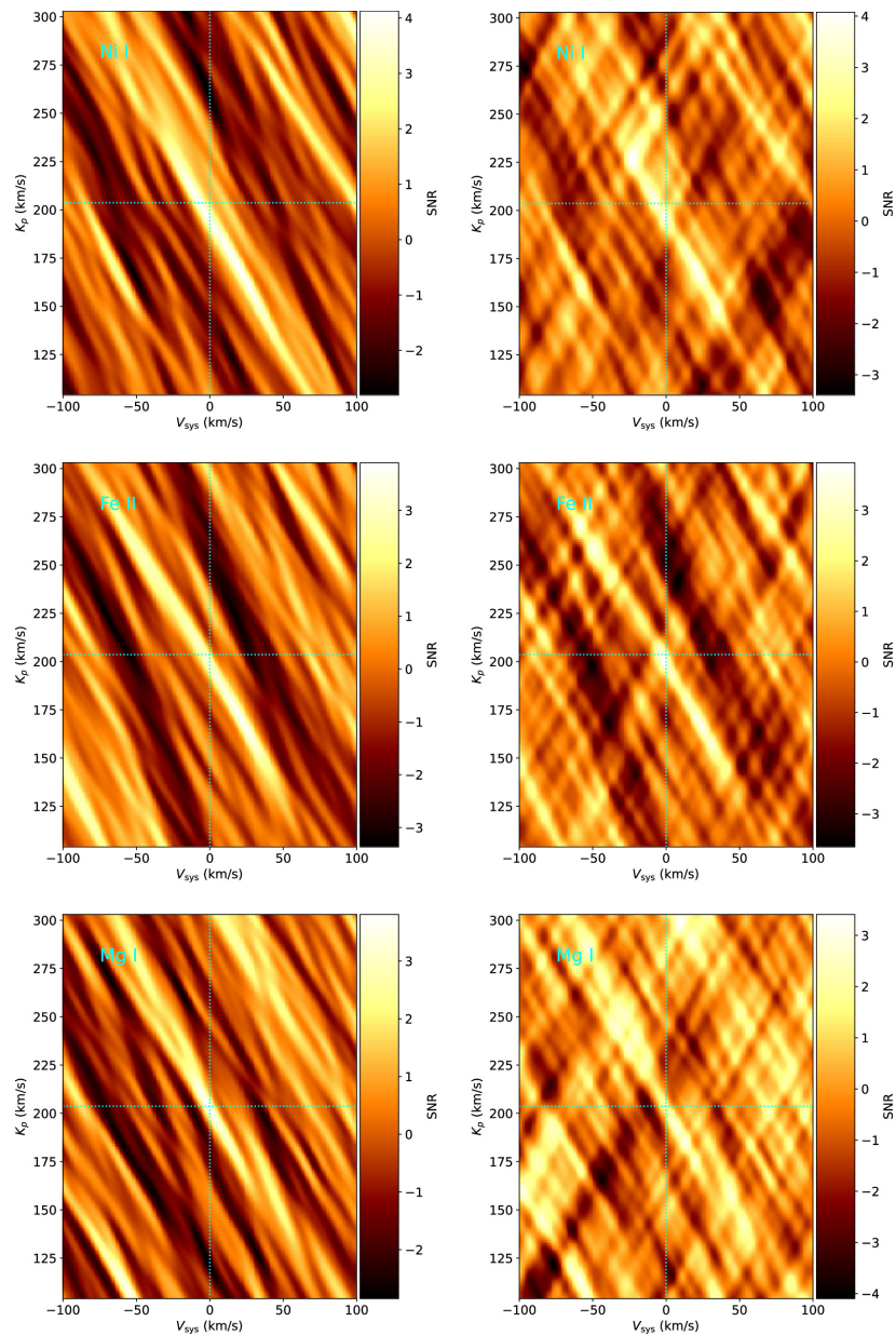
Figure 5. from Sydney Petz et al 2025 Astron. J. 169 doi:10.3847/1538-3881/adc411 https://dx.doi.org/10.3847/1538-3881/adc411 © 2025. The Author(s). Published by the American Astronomical Society.
