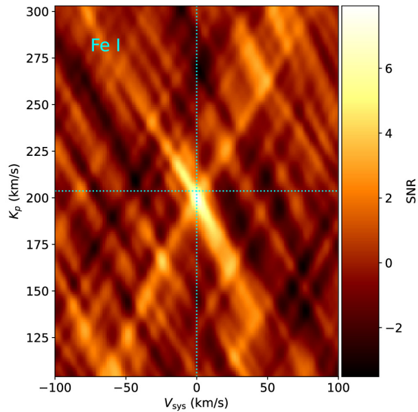
Figure 4. from Sydney Petz et al 2025 Astron. J. 169 doi:10.3847/1538-3881/adc411 https://dx.doi.org/10.3847/1538-3881/adc411 © 2025. The Author(s). Published by the American Astronomical Society.
