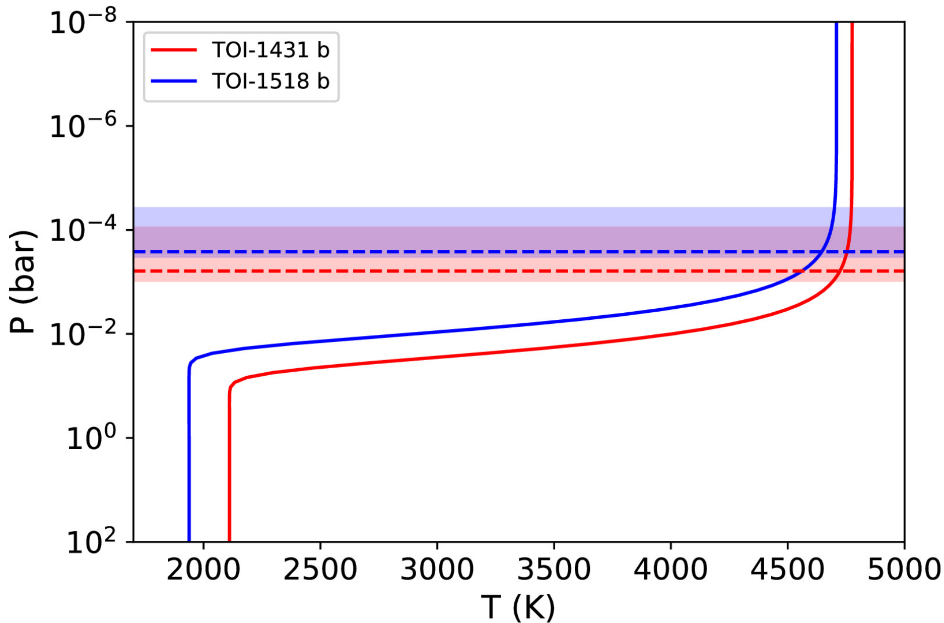
Figure 2. from Sydney Petz et al 2025 Astron. J. 169 doi:10.3847/1538-3881/adc411 https://dx.doi.org/10.3847/1538-3881/adc411 © 2025. The Author(s). Published by the American Astronomical Society.
