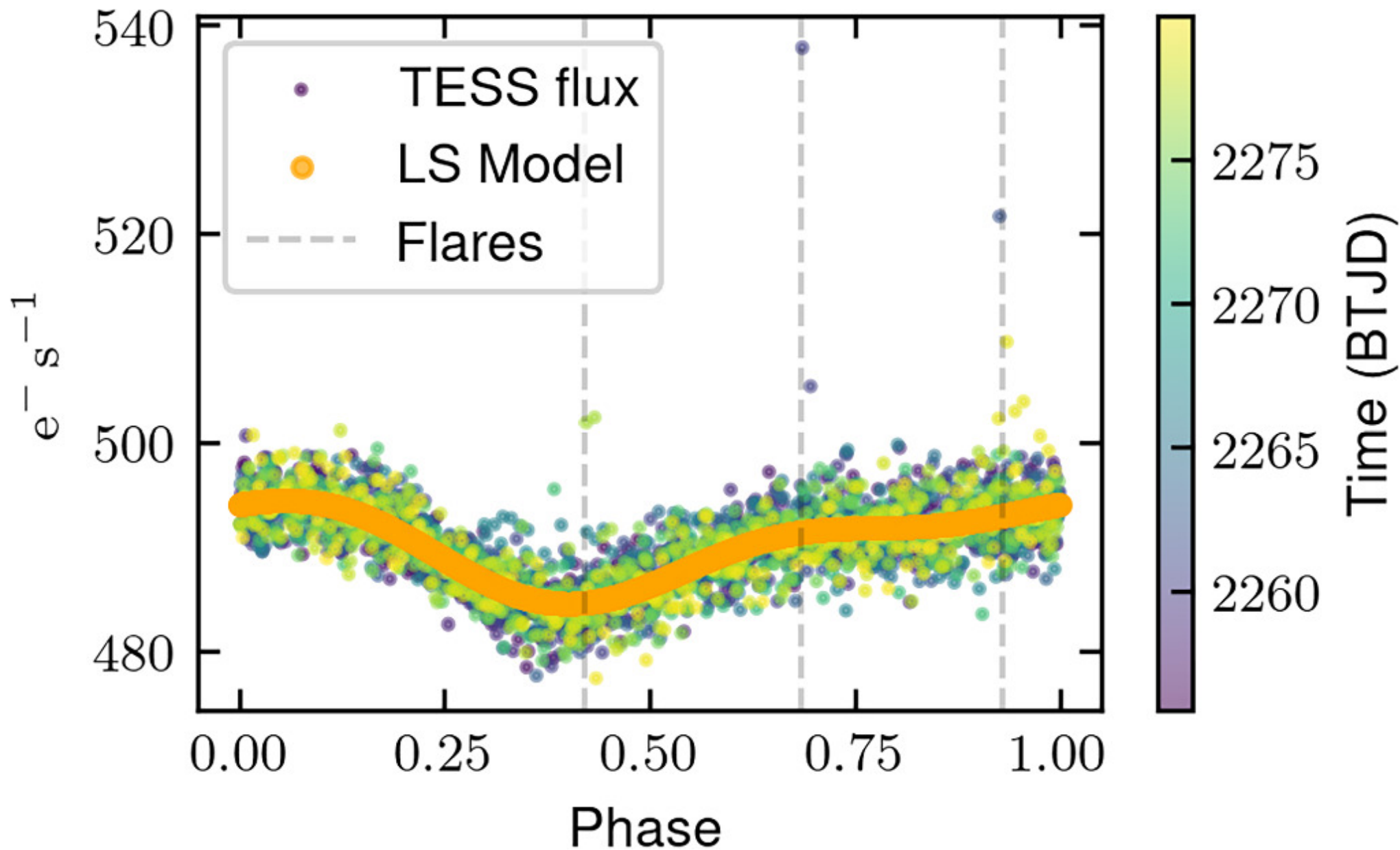
Figure 7. from Hank Corbett et al 2025 Astron. J. 169 doi:10.3847/1538-3881/adc391 https://dx.doi.org/10.3847/1538-3881/adc391 © 2025. The Author(s). Published by the American Astronomical Society.
