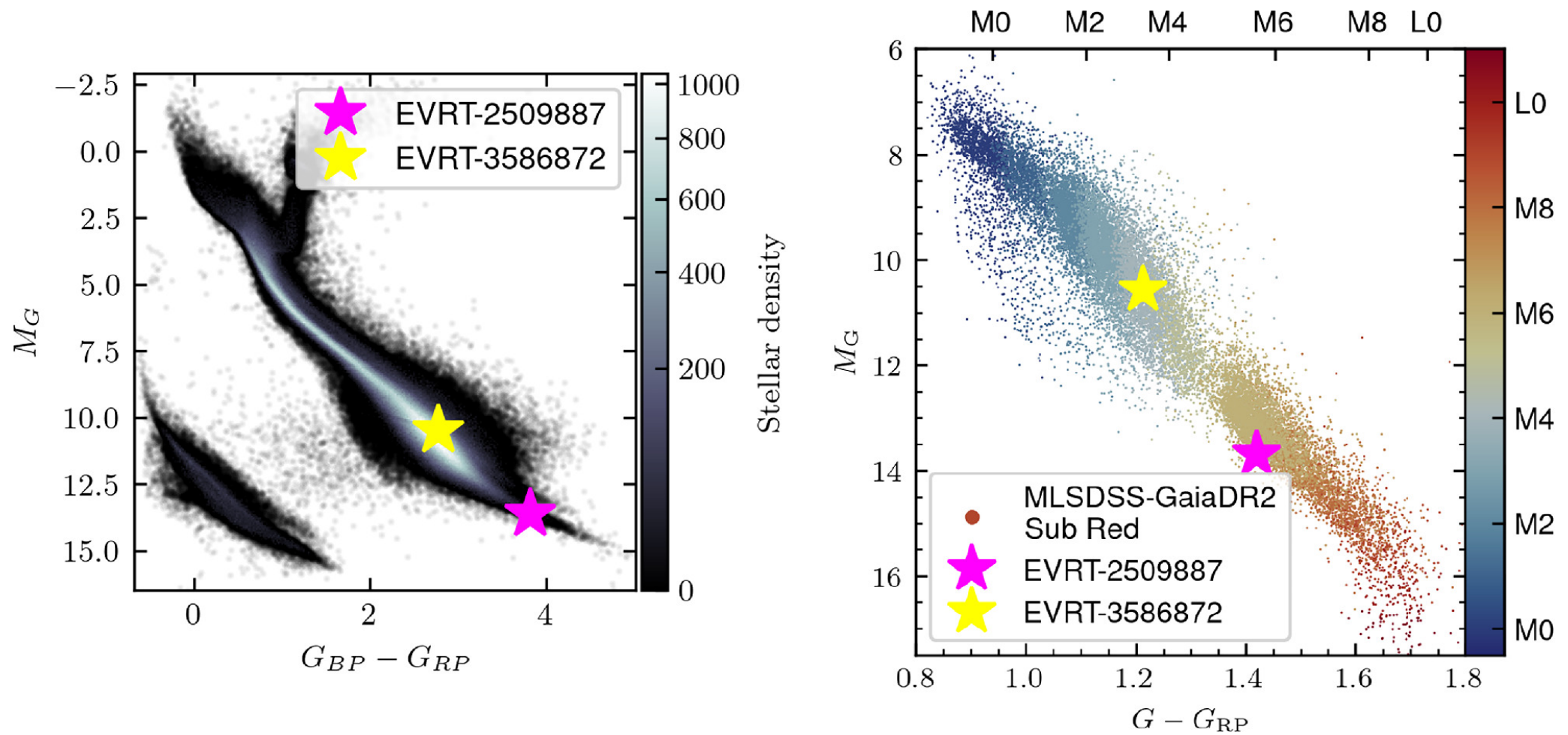
Figure 6. from Hank Corbett et al 2025 Astron. J. 169 doi:10.3847/1538-3881/adc391 https://dx.doi.org/10.3847/1538-3881/adc391 © 2025. The Author(s). Published by the American Astronomical Society.
