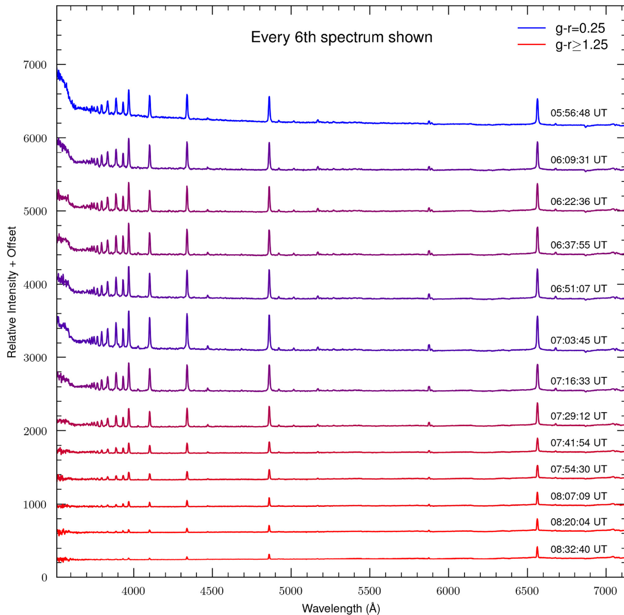
Figure 3. from Hank Corbett et al 2025 Astron. J. 169 doi:10.3847/1538-3881/adc391 https://dx.doi.org/10.3847/1538-3881/adc391 © 2025. The Author(s). Published by the American Astronomical Society.
