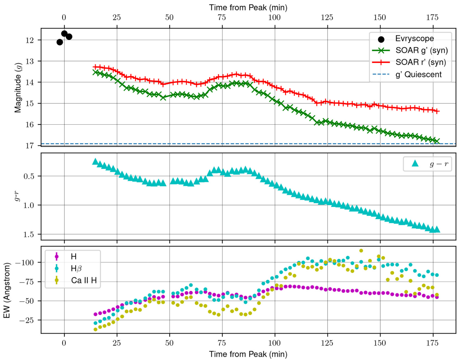
Figure 2. from Hank Corbett et al 2025 Astron. J. 169 doi:10.3847/1538-3881/adc391 https://dx.doi.org/10.3847/1538-3881/adc391 © 2025. The Author(s). Published by the American Astronomical Society.
