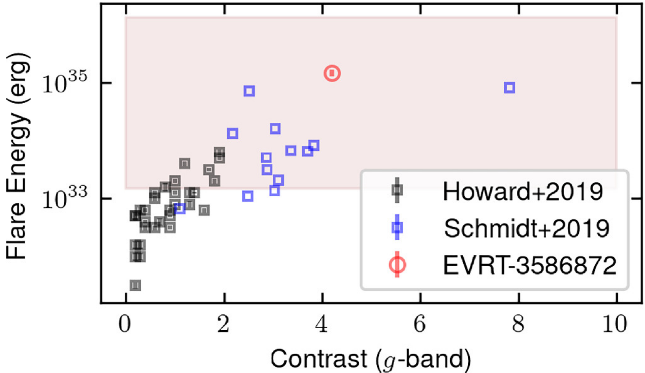
Figure 13. from Hank Corbett et al 2025 Astron. J. 169 doi:10.3847/1538-3881/adc391 https://dx.doi.org/10.3847/1538-3881/adc391 © 2025. The Author(s). Published by the American Astronomical Society.
