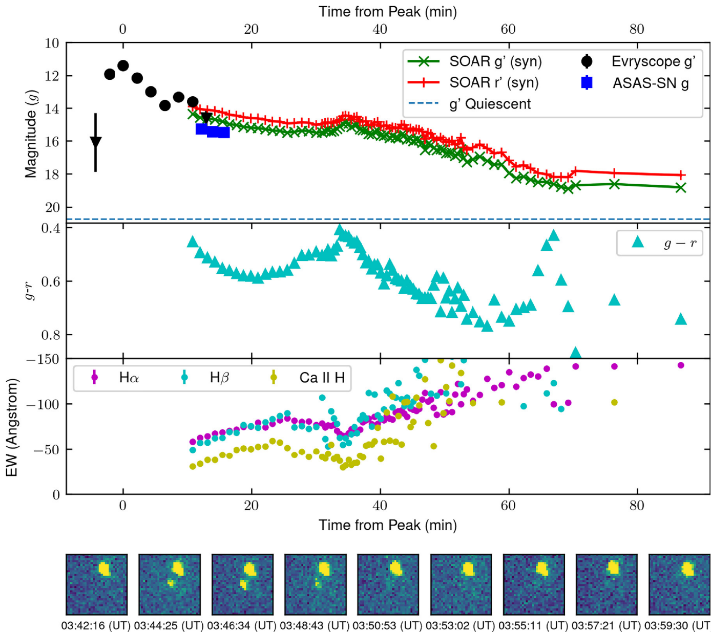
Figure 1. from Hank Corbett et al 2025 Astron. J. 169 doi:10.3847/1538-3881/adc391 https://dx.doi.org/10.3847/1538-3881/adc391 © 2025. The Author(s). Published by the American Astronomical Society.
