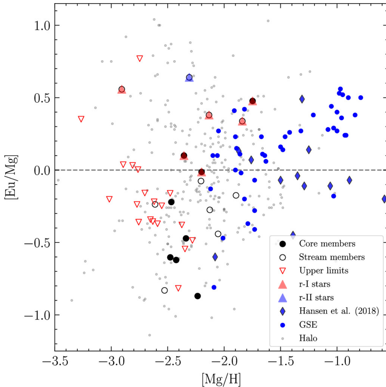
Figure 9. from Xiaowei Ou et al 2025 Astron. J. 169 doi:10.3847/1538-3881/adc126 https://dx.doi.org/10.3847/1538-3881/adc126 © 2025. The Author(s). Published by the American Astronomical Society.
