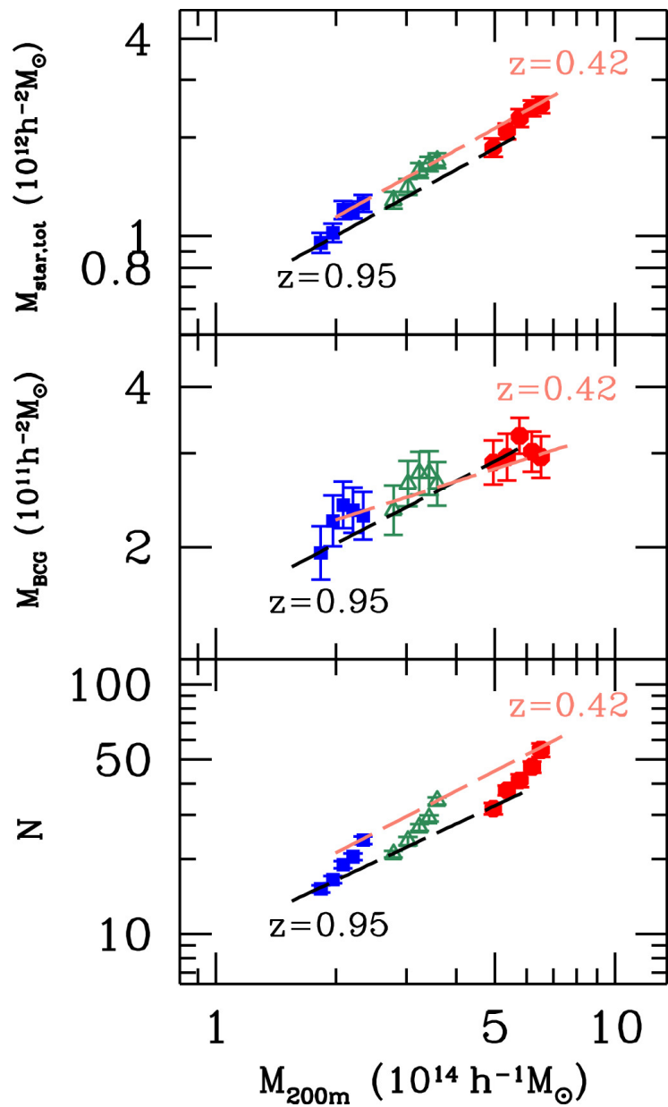
Figure 7. from Yen-Ting Lin et al 2025 Astron. J. 169 doi:10.3847/1538-3881/adc0f8 https://dx.doi.org/10.3847/1538-3881/adc0f8 © 2025. The Author(s). Published by the American Astronomical Society.
