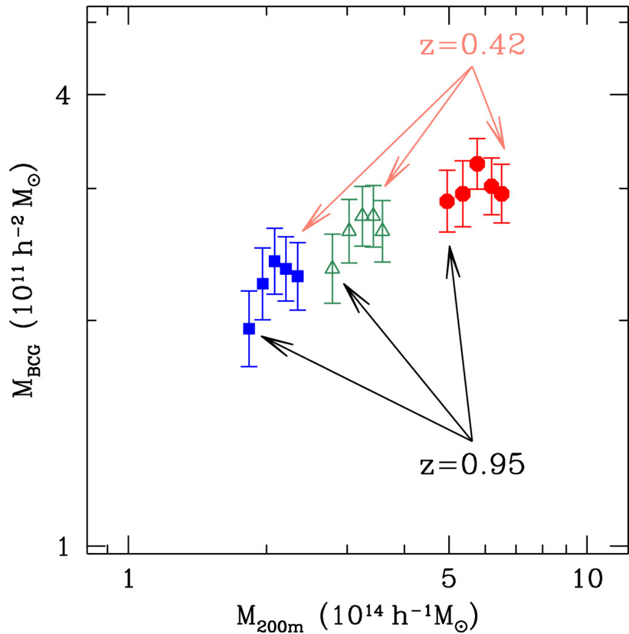
Figure 5. from Yen-Ting Lin et al 2025 Astron. J. 169 doi:10.3847/1538-3881/adc0f8 https://dx.doi.org/10.3847/1538-3881/adc0f8 © 2025. The Author(s). Published by the American Astronomical Society.
