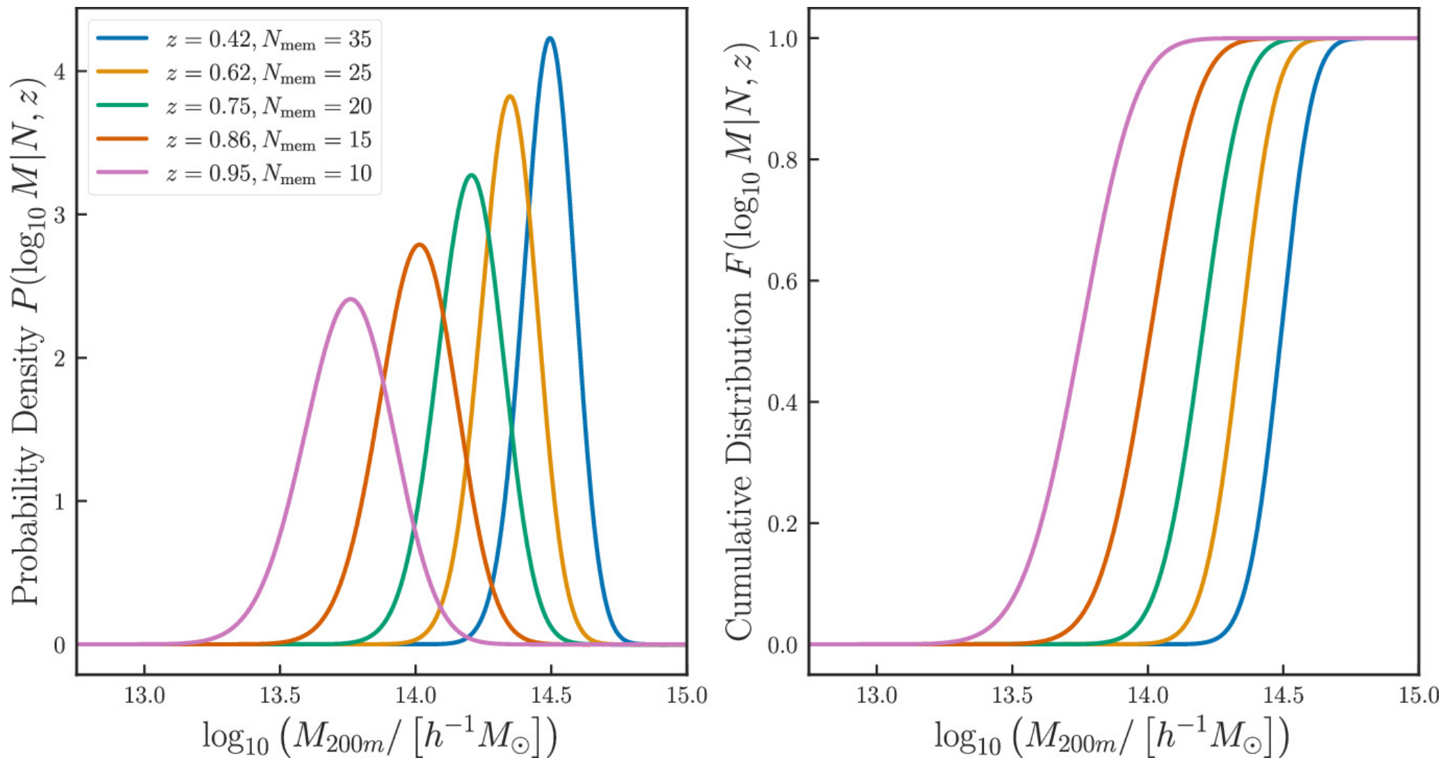
Figure 3. from Yen-Ting Lin et al 2025 Astron. J. 169 doi:10.3847/1538-3881/adc0f8 https://dx.doi.org/10.3847/1538-3881/adc0f8 © 2025. The Author(s). Published by the American Astronomical Society.
