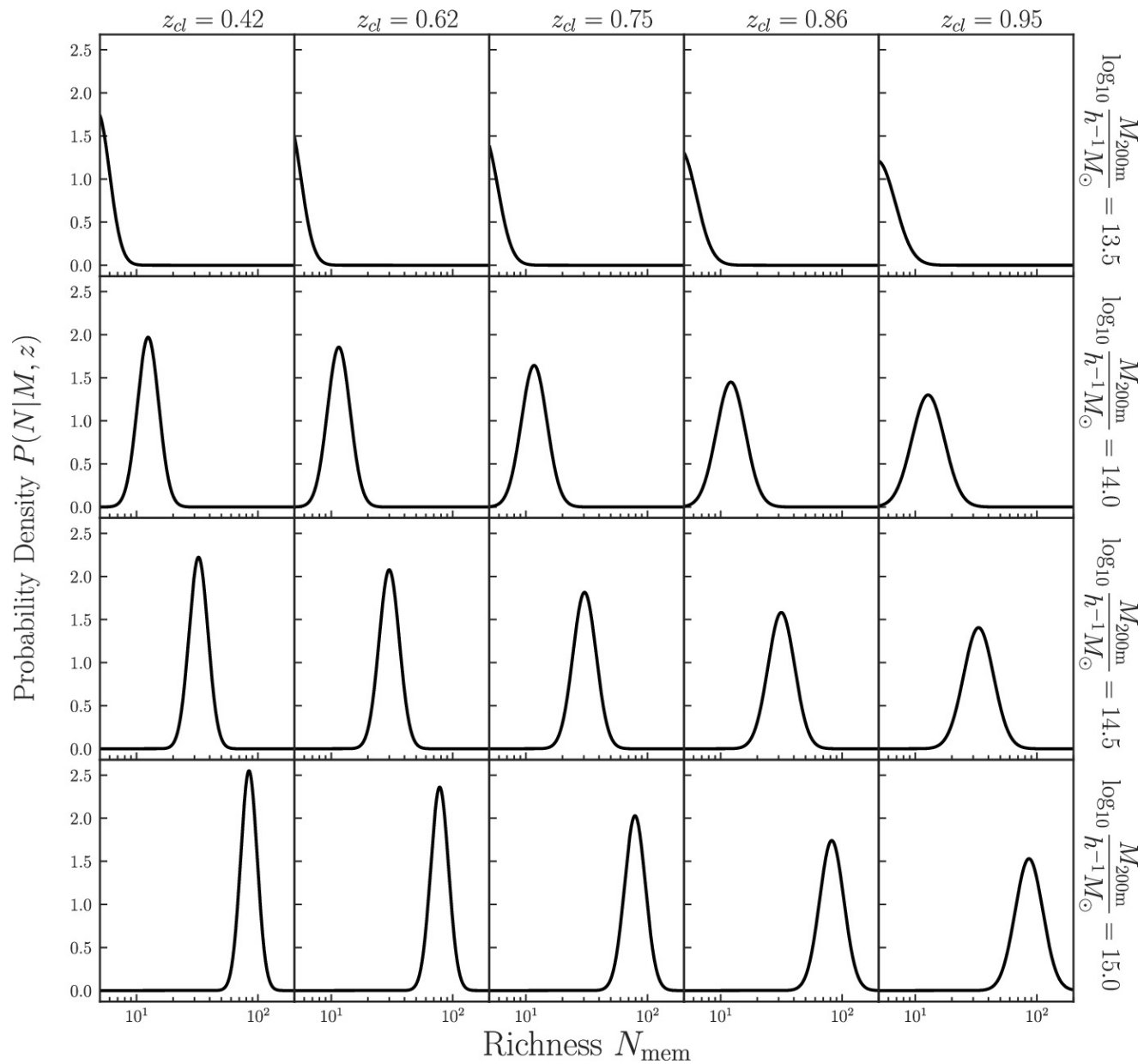
Figure 2. from Yen-Ting Lin et al 2025 Astron. J. 169 doi:10.3847/1538-3881/adc0f8 https://dx.doi.org/10.3847/1538-3881/adc0f8 © 2025. The Author(s). Published by the American Astronomical Society.
