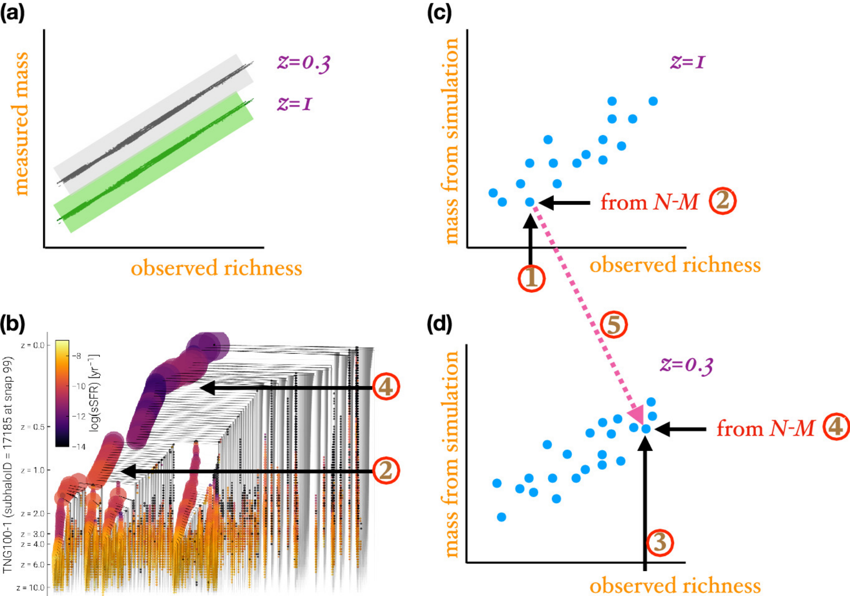
Figure 1. from Yen-Ting Lin et al 2025 Astron. J. 169 doi:10.3847/1538-3881/adc0f8 https://dx.doi.org/10.3847/1538-3881/adc0f8 © 2025. The Author(s). Published by the American Astronomical Society.
