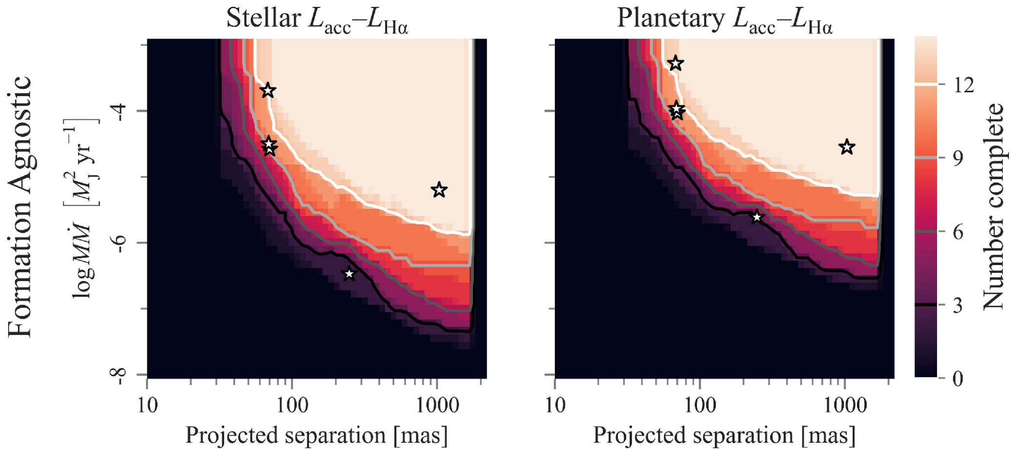
Figure 4. from Cailin Plunkett et al 2025 Astron. J. 169 doi:10.3847/1538-3881/adc09d https://dx.doi.org/10.3847/1538-3881/adc09d © 2025. The Author(s). Published by the American Astronomical Society.
