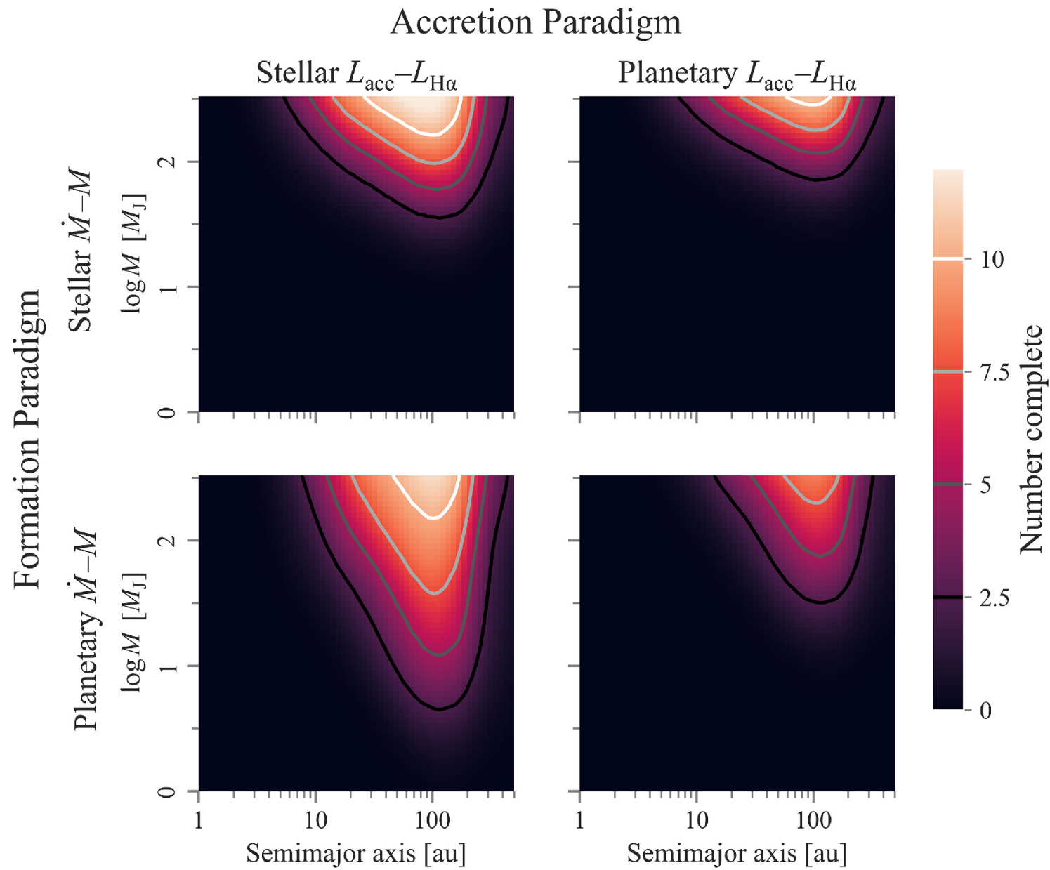
Figure 2. from Cailin Plunkett et al 2025 Astron. J. 169 doi:10.3847/1538-3881/adc09d https://dx.doi.org/10.3847/1538-3881/adc09d © 2025. The Author(s). Published by the American Astronomical Society.
