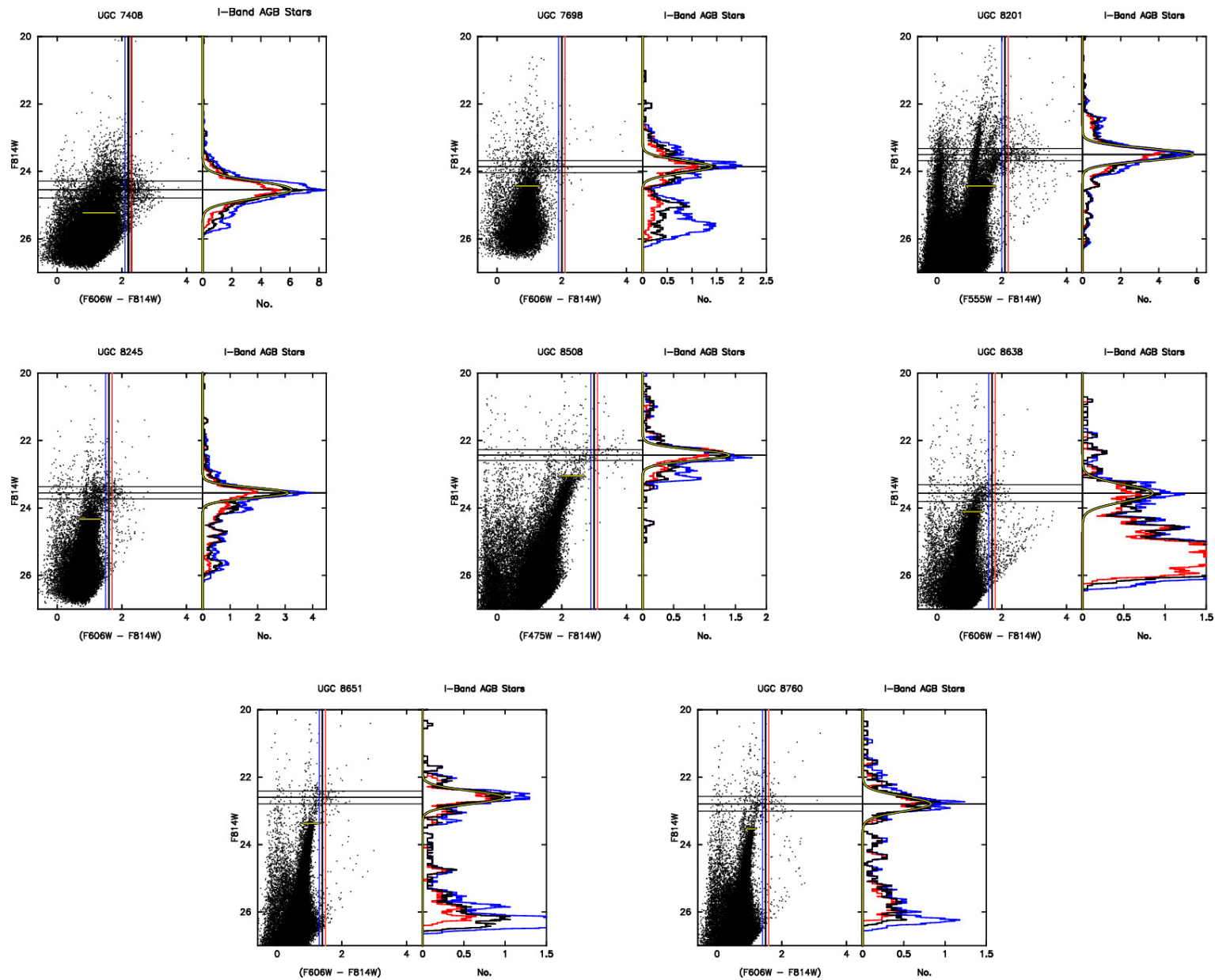
Figure 6. from Wendy L. Freedman et al 2025 Astron. J. 169 doi:10.3847/1538-3881/adbf97 https://dx.doi.org/10.3847/1538-3881/adbf97 © 2025. The Author(s). Published by the American Astronomical Society.
